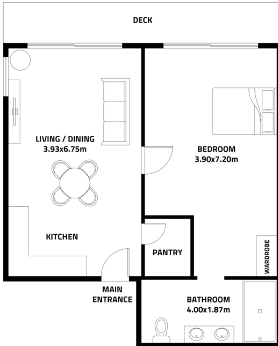
FLOOR PLAN
